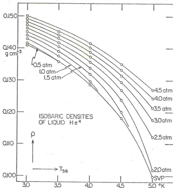
FIG. 2. Isobaric densities of liquid \text{He}^4 as a function of temperature for pressures up to 4.5 atmospheres.
